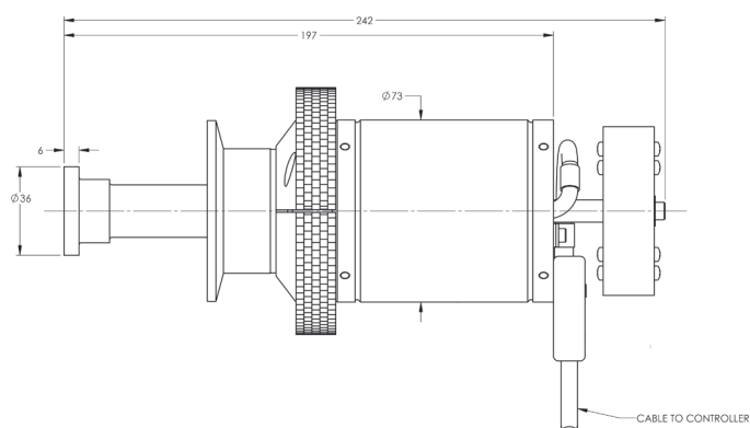
MT Cryocooler with Air Fins
