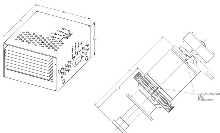
MT Cryocooler with Air Fins
